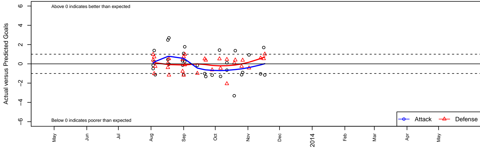
So Cal Blues Otto G00 Dots are actual minus expected GF (blue circles) and GA (red triangles). Blue line is smoothed change in attack strength. Red is smoothed change in defense strength.
